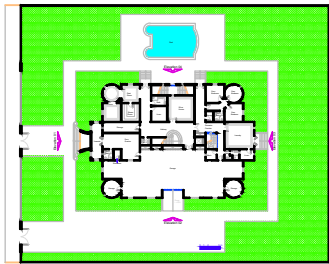
Lower Floor Plan A = 617.26 m 2
